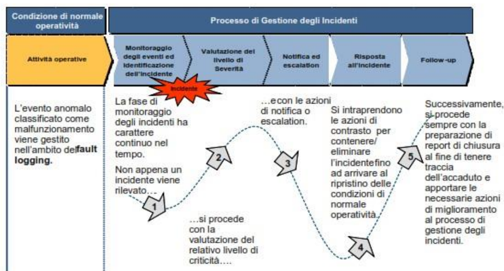
Figura 15 Incident Management
