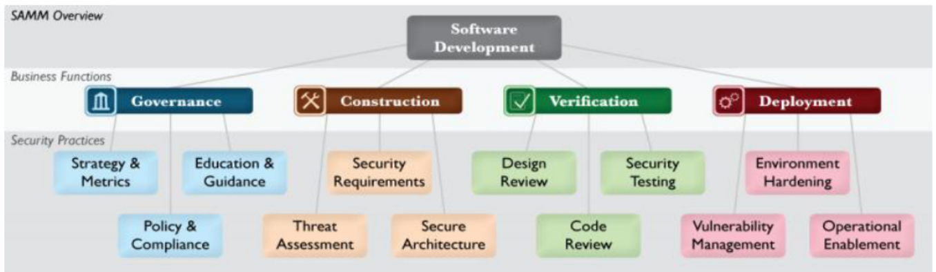
Figura 14 - SAMM Structure
